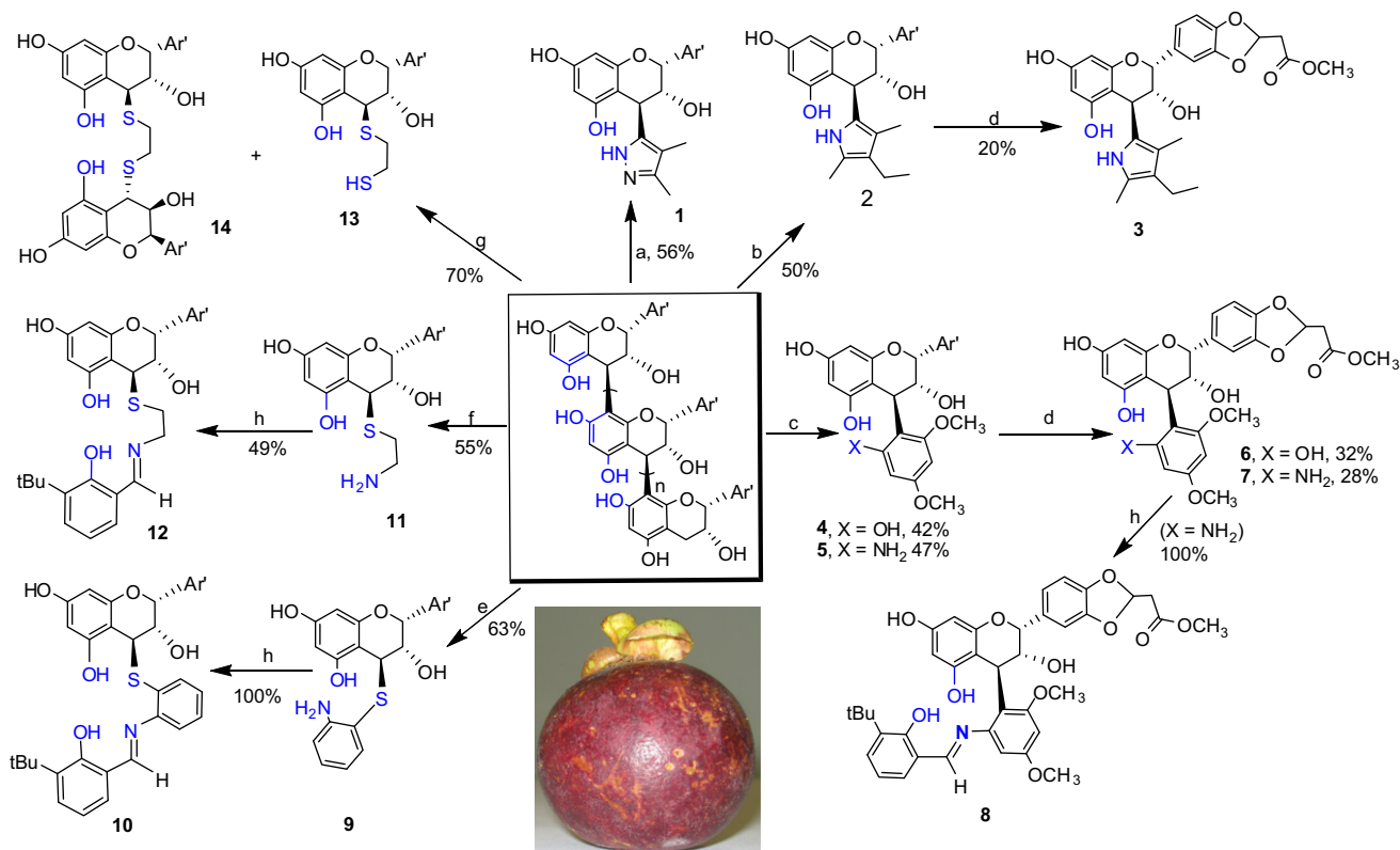
Scheme 1. From oligomeric proanthocyanidins ( n = 2-50 ) in mangosteen peels (inset) to multidentate ligands, (Ar' = 3,4-dihydroxyphenyl). Acid mediated depolymerization conditions are 0.22% HCl in CH 3 OH, 45 °C, 2–8 h. (a) 2,3-Dimethylpyrazole; (b) 3-ethyl-2,4-dimethylpyrrole; (c) 3,5-dimethoxyphenol (for 4 ), or 3,5-dimethoxyaniline (for 5 ); (d) 4-( N,N -dimethylamino)pyridine, HCCCOCH 3 CH 3 CN, rt, 12 h; (e) o -thioaniline; (f) cysteamine; (g) 1,2-dithioethane; (h) 3- tert -butylsalicylaldehyde, CH 3 OH, AcOH, 1 drop, rt. Percentage conversion was determined by HPLC.
